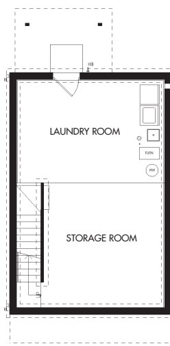
BASEMENT PLAN
